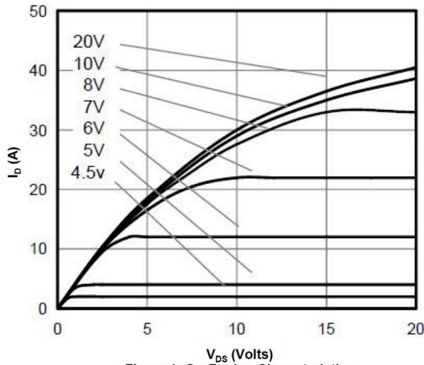
Figure 1: On-Region Characteristics
